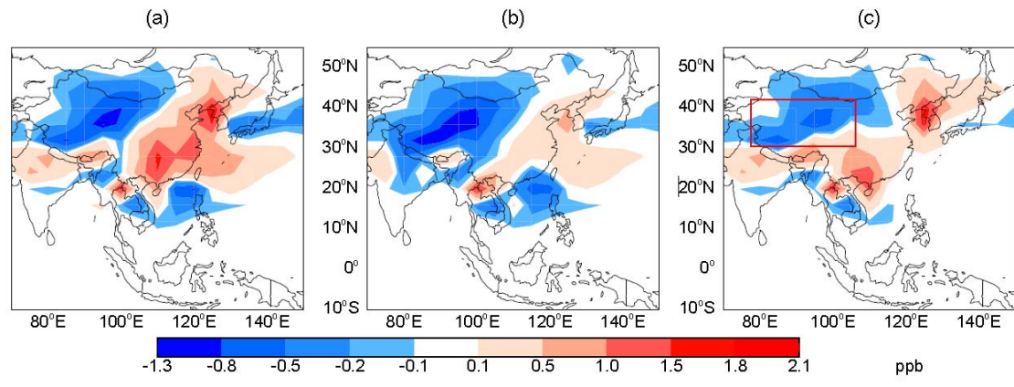
5 6 Figure 6. (a) The summer-mean difference in the effect of the 2000-2050 Chinese emission 7 change on surface ozone between the 2000 and 2050 climate; (b) same as a, but without the 8 changes in biogenic emissions of VOCs as a function of climate change; (c) same as a, but 9 without the changes in the anthropogenic emissions over Central East China (CEC). The red 10 rectangular region in (c) indicates West China.
