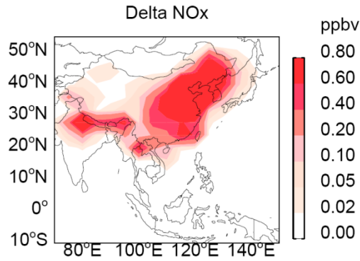
2 Figure 7. The effect on annual-mean surface \text{NO}_x mixing ratios in the 2000 climate brought 3 merely by the 2000-2050 changes of Chinese anthropogenic emissions.
