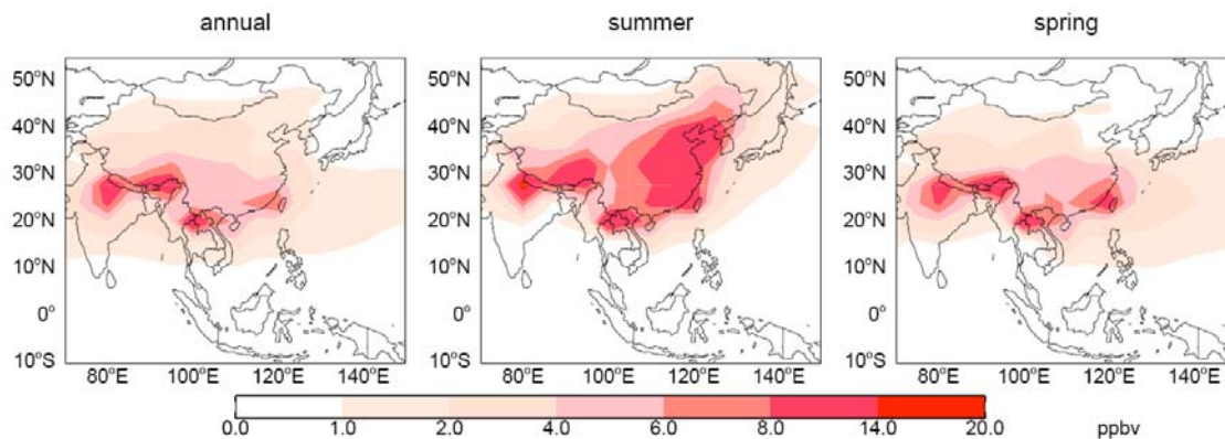
4 5 Figure 4. The effect of the 2000-2050 changes in Chinese anthropogenic emissions only on 6 surface ozone: (a) annual-mean, (b) summer; (c) spring.
