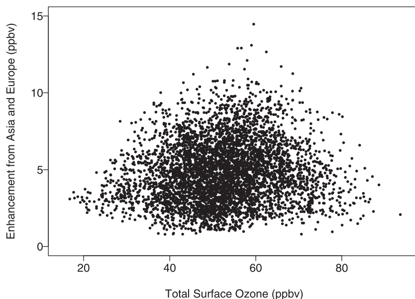
Figure 15. Enhancement to afternoon background O 3 in surface air over the United States due to anthropogenic emissions in Asia and Europe, plotted as a function of total O 3 concentrations in the model surface layer. Points represent daily afternoon (1300–1700 LT) model values for the ensemble of days in June–August 1995 for all U.S. grid squares.
